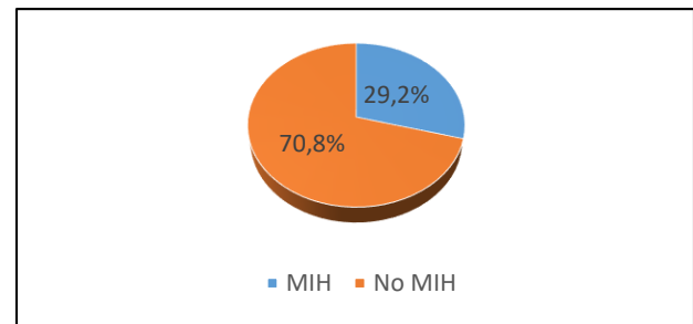
Figure 2. MIH distribution
